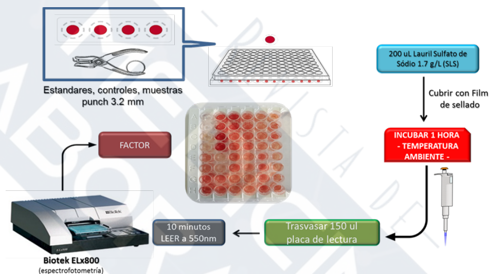
Figure 1. Schematic diagram of the hematocrit estimation technique.
